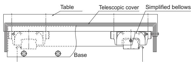
Fig.2 Example of Mounting the Simplified Bellows
