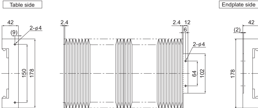
Fig.4 External Dimensions of the Bellows
