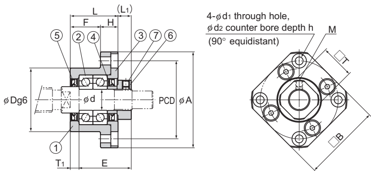
Mounting method A
